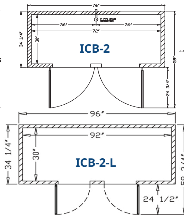
TOP VIEWS
