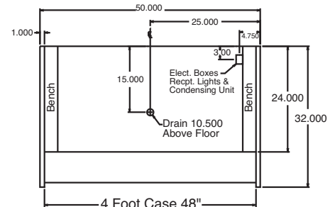
PLAN VIEWS
