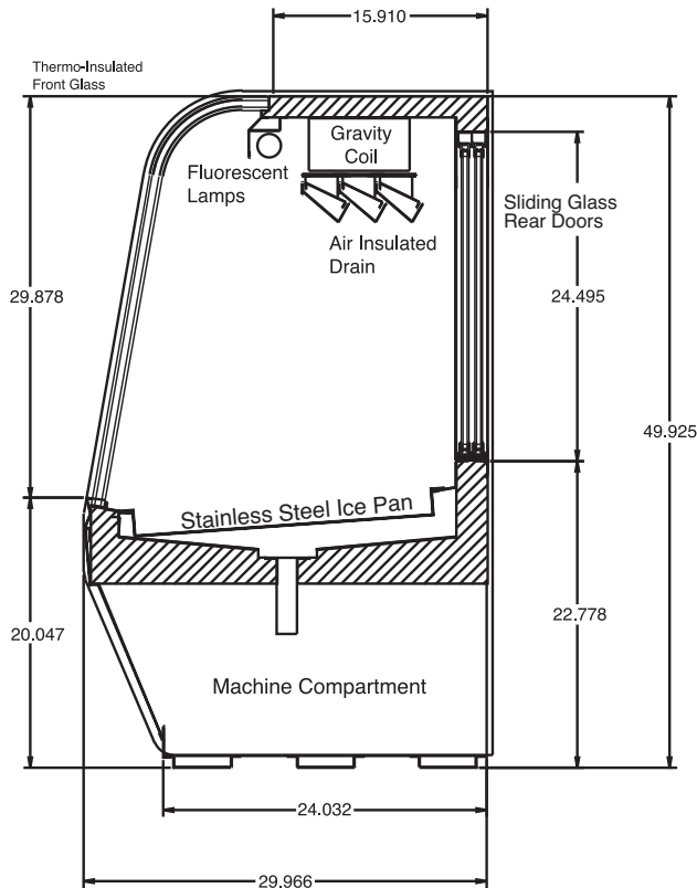
CROSS SECTION
