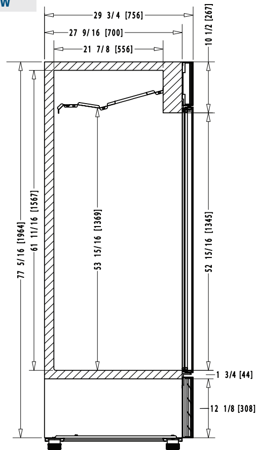
HEADER DIMS
