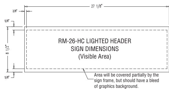
HEADER DIMS
